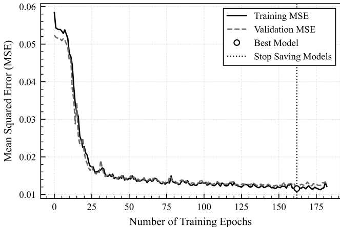
Learning Curve of GRU Model for SolarPlant-1 (Gyeongju)
